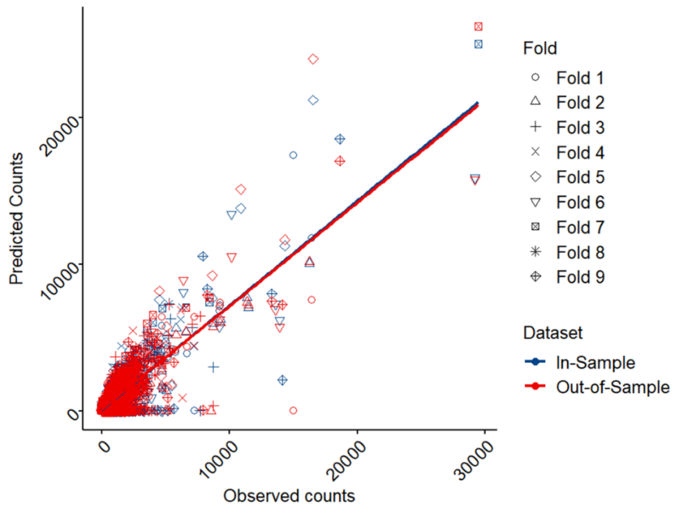
Figure 2. Scatter plots of model cross validations for in-sample and out-of-sample test datasets
